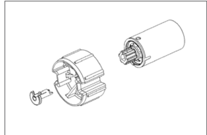
Picture 2: Coupling locking device*
